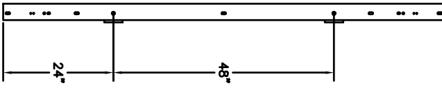
WALL COAX BRACKET SPACING
